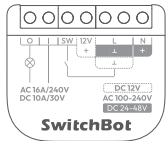
SwitchBot Relay Switch 1
