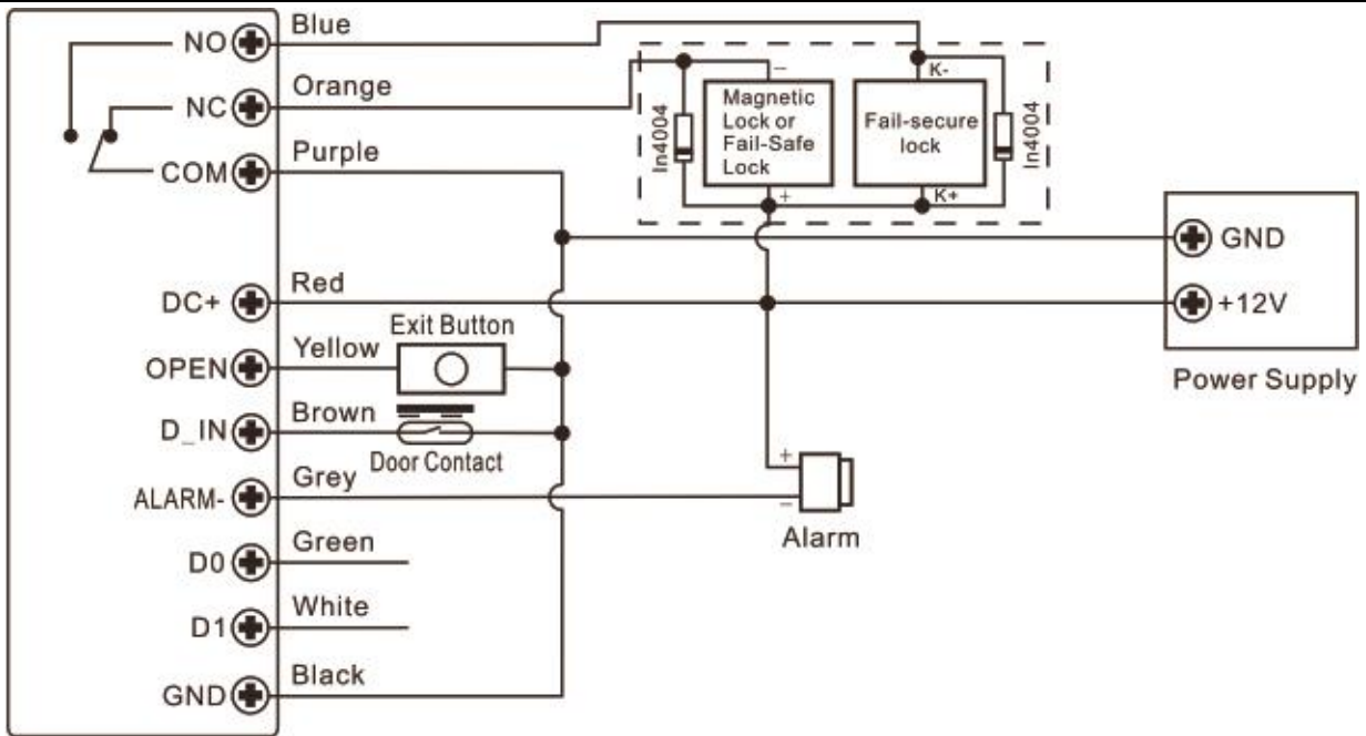
fig.1 Standard wiring diagram
